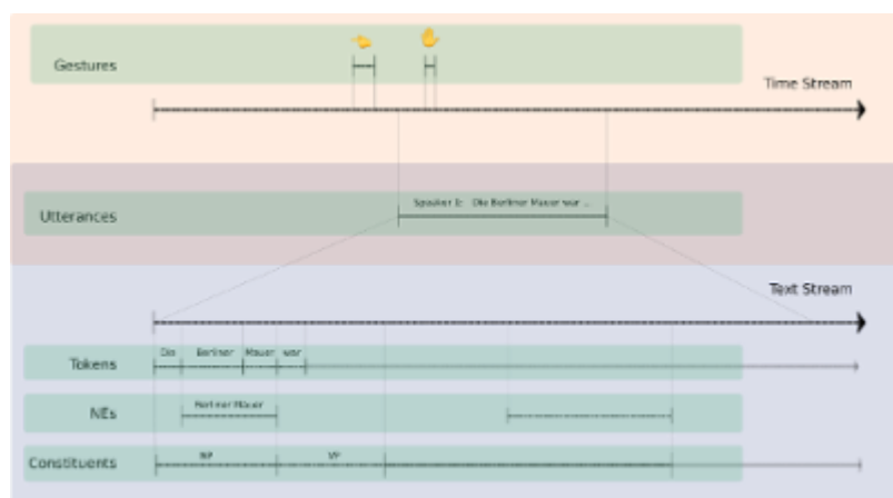
Fig 1. Data representation on virtual alignment streams
